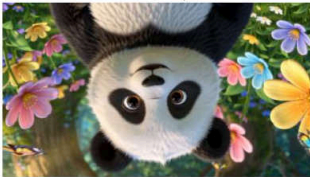
Vertical Flip
